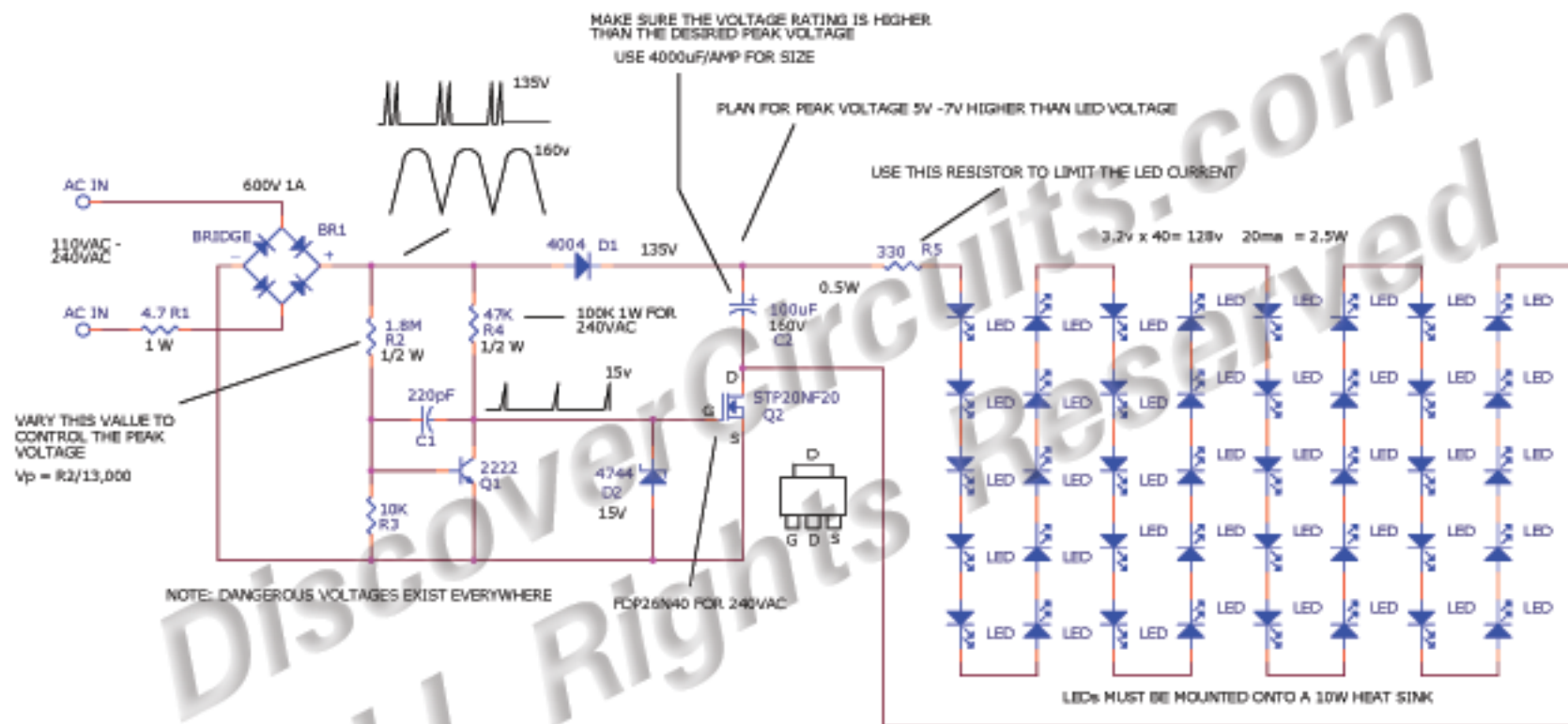
AC LINE POWERED 40 WHITE LED SERIES STRING DRIVER
