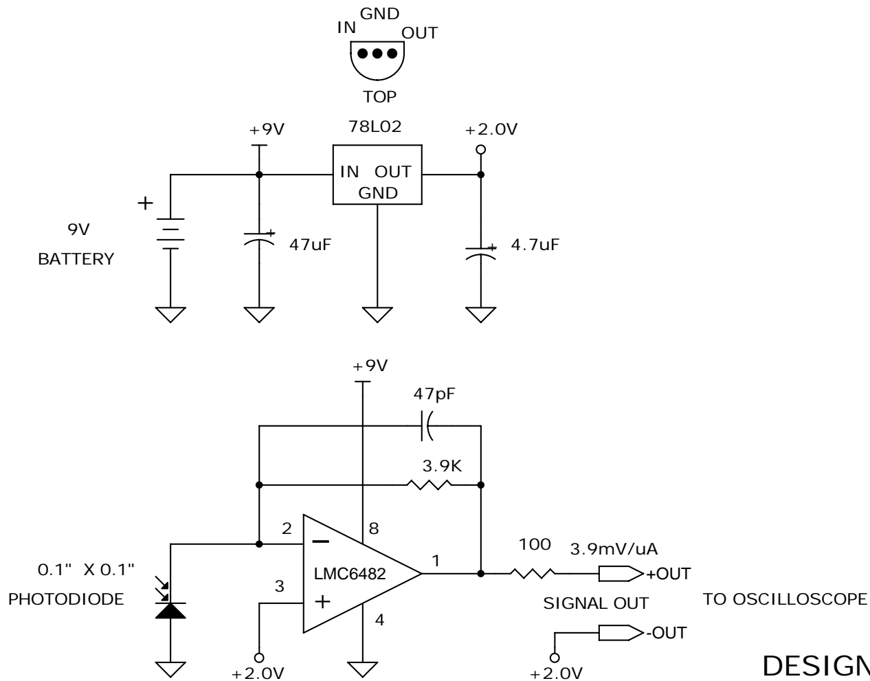
LIGHT MONITOR Bandwidth = 500KHz
