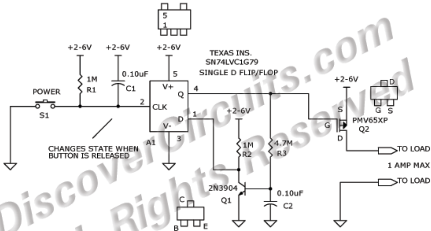
PUSH-ON, PUSH-OFF SWITCH CIRCUIT
