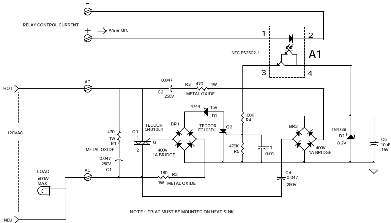
OPTICALLY ISOLATED SOLID STATE RELAY 50uA CONTROL CURRENT
