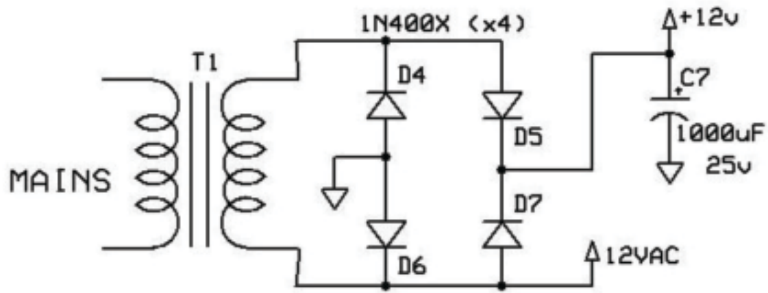
Figure 1. Power supply section
