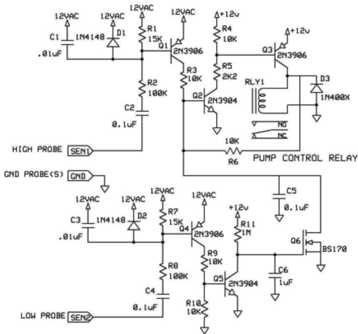
Figure 2. Corrosion resistant sump pump controller
