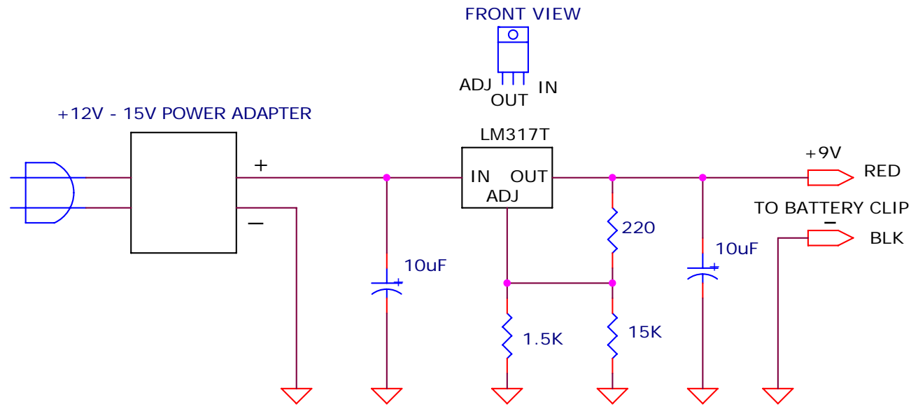
9V BATTERY ELIMINATOR
