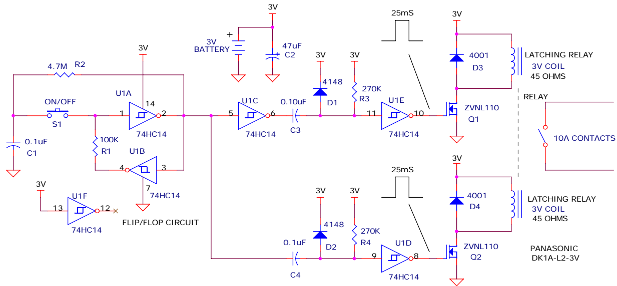
ON/OFF SWITCH WITH LATCHING RELAY
