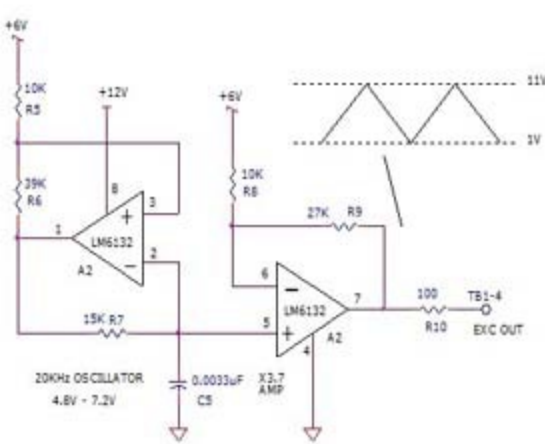
12V TOUCH SWITCH EXCITATION SIGNAL GENERATOR
