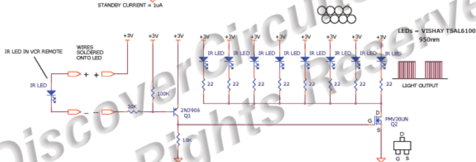
TV-VCR REMOTE REPEATER
