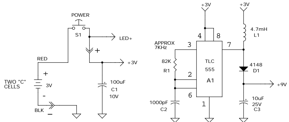
VOLTAGE CONVERTER
