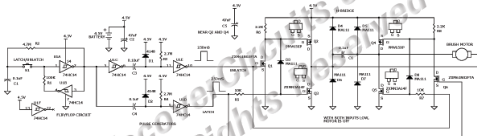
PULSED CW & CCW MOTOR DRIVER
