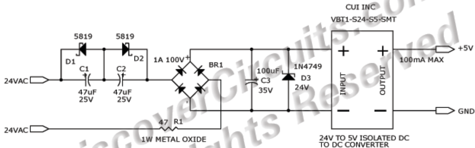
MINIATURE 24VAC POWERED ISOLATED 5V POWER SUPPLY
