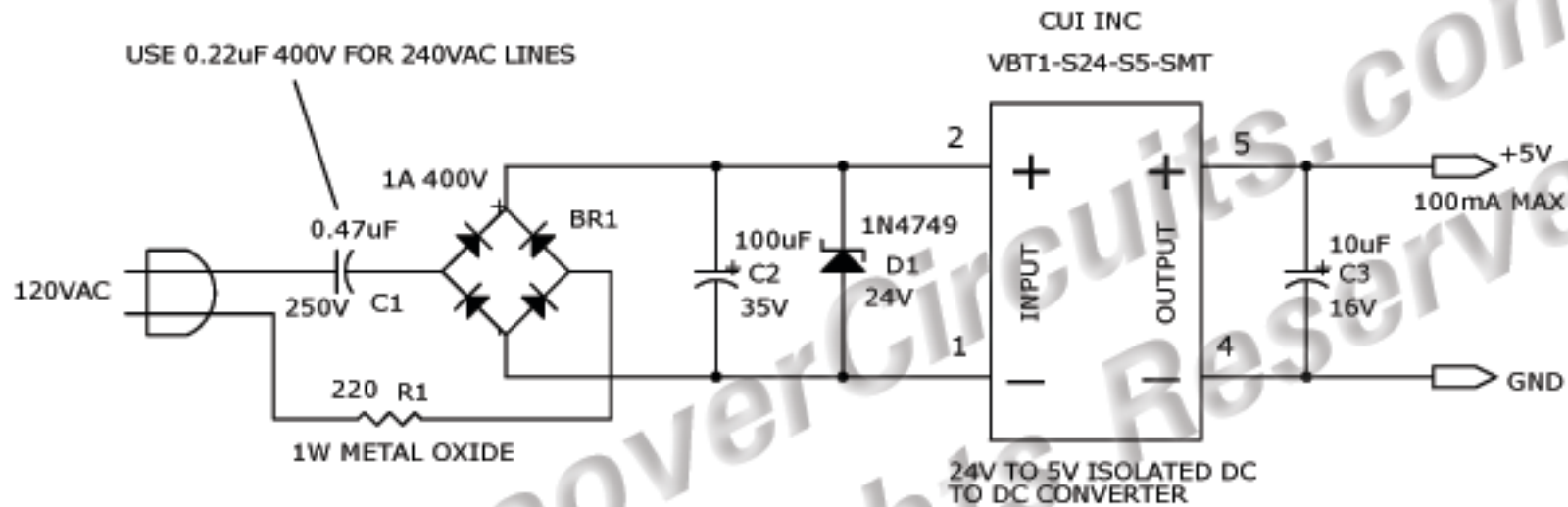
MINIATURE LINE POWERED ISOLATED 5V POWER SUPPLY
