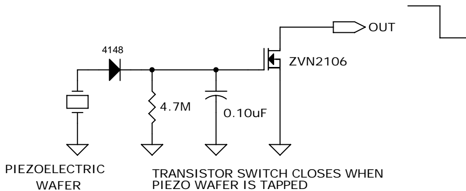
PIEZOELECTRIC TRIGGERED SWITCH
